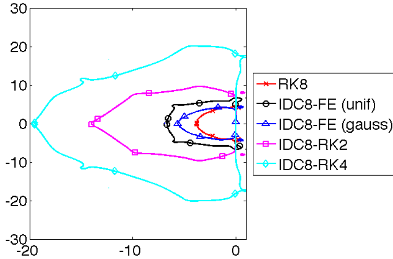
(a) 8 th Order Methods
