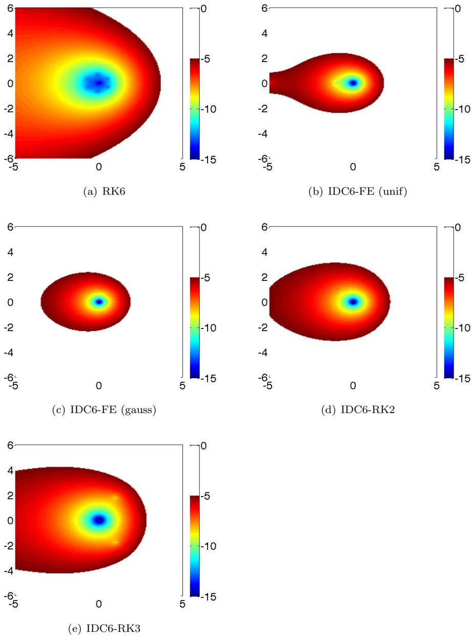
FIG. 4.3. Accuracy plots for various sixth order RK and IDC methods are generated using \approx 60 function evaluations. The RK6 method has a larger accuracy region. Also, observe that the accuracy regions for the IDC methods increase with the order of the embedded integrator.
