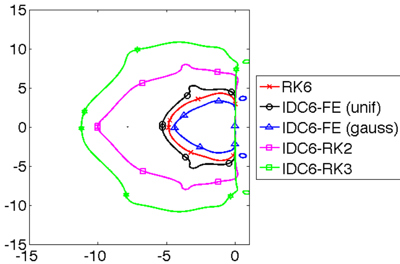
(b) 6 th Order Methods
