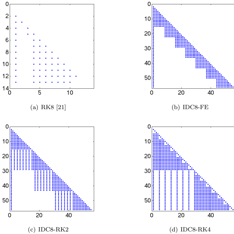
FIG. 4.1. The sparsity structure of an RK8 [21] Butcher tableau and various IDC8 butcher tables. The block structure for the IDC weights are evident; for example, IDC8-RK2 shows the prediction loop, and the subsequent three correction loops.
