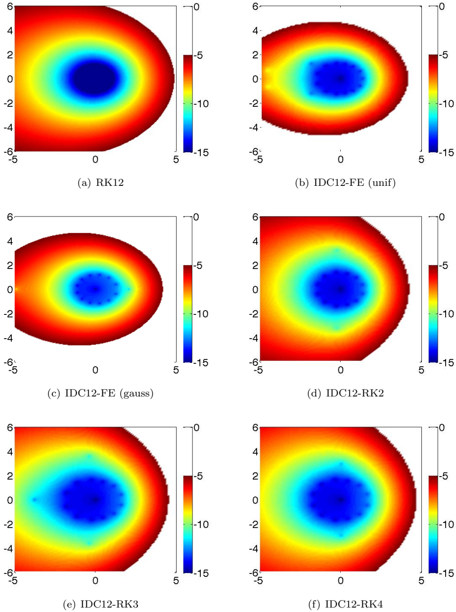
FIG. 4.5. The accuracy plots for various twelfth order RK and IDC methods are generated after \approx 132 function evaluations. The accuracy region for IDC12-RK3 and IDC12-RK4 appear larger than the classically known RK12 scheme.
