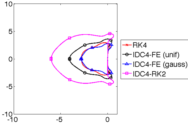
(a) 4 th Order Methods
