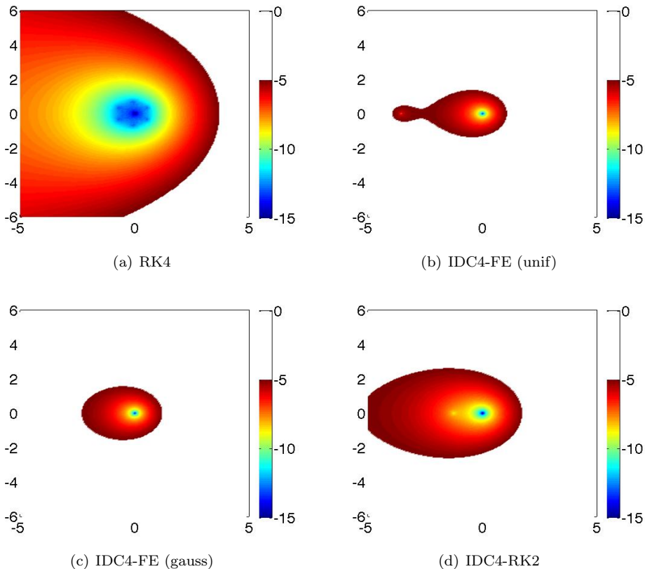
FIG. 4.2. Accuracy plots for various fourth order RK and IDC methods. Each plot was generated after 48 function evaluations. The RK_4 method is vastly superior to the IDC methods.
