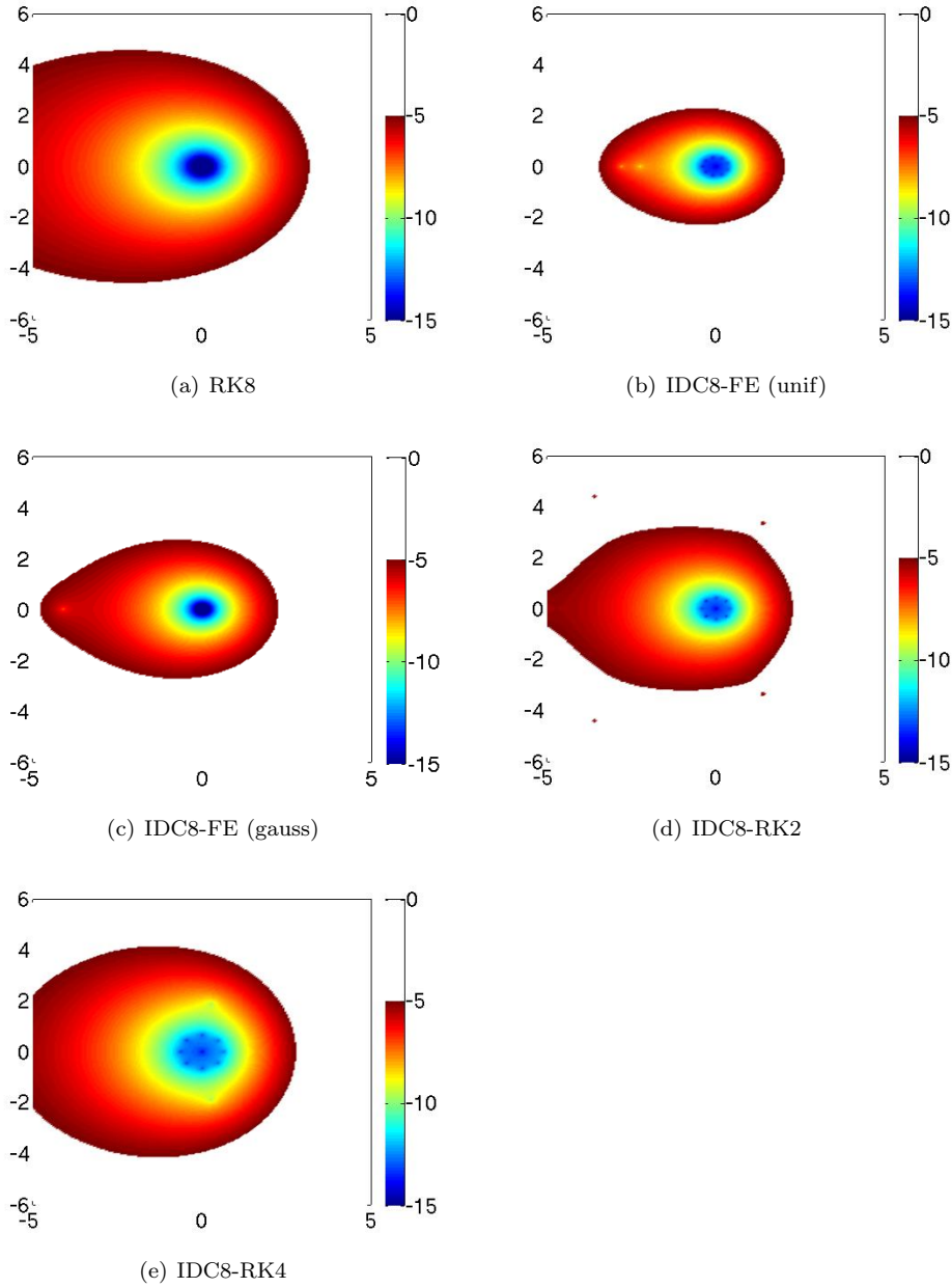
FIG. 4.4. The accuracy plots for various eighth order RK and IDC methods are generated after \approx 56 function evaluations. Notice that accuracy regions for IDC methods get larger as the order of the low order integrator is increased. The accuracy region for IDC8-RK4 is comparable to the accuracy region for RK8, consistent with the efficiency analysis.
