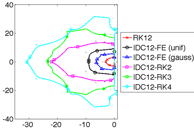
(b) 12 th Order Methods
